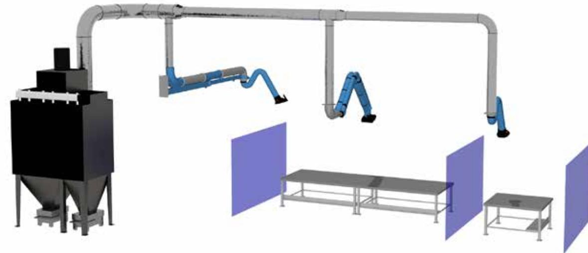
Typical MCP SmartFilter fume or dust collection solution featuring multiple extraction points, variety of extraction arms, QF duct, integral mounted fan.
